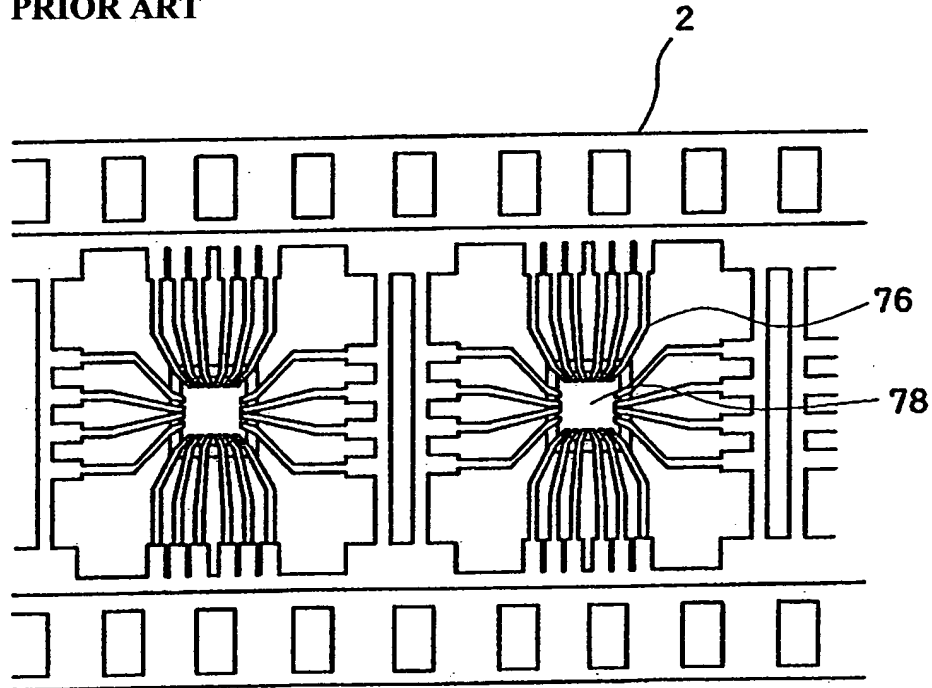
FIG. 7 PRIOR ART
